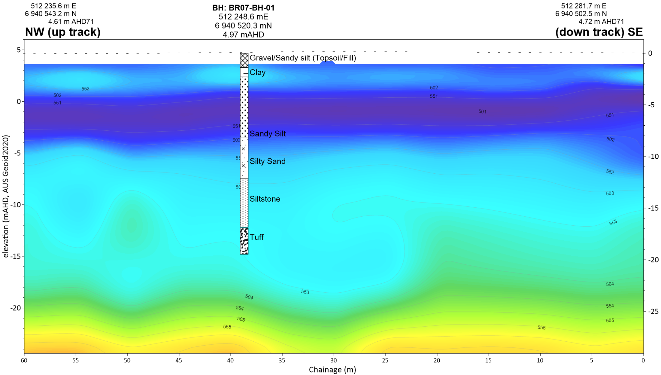
Seismic Line MASW AU-GP 143-1
